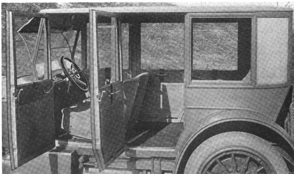
INTERIOR VIEW OF SPORTING ENCLOSED DRIVE BREWSTER
